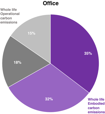
Speculative office building with Cat A fit out; central London
