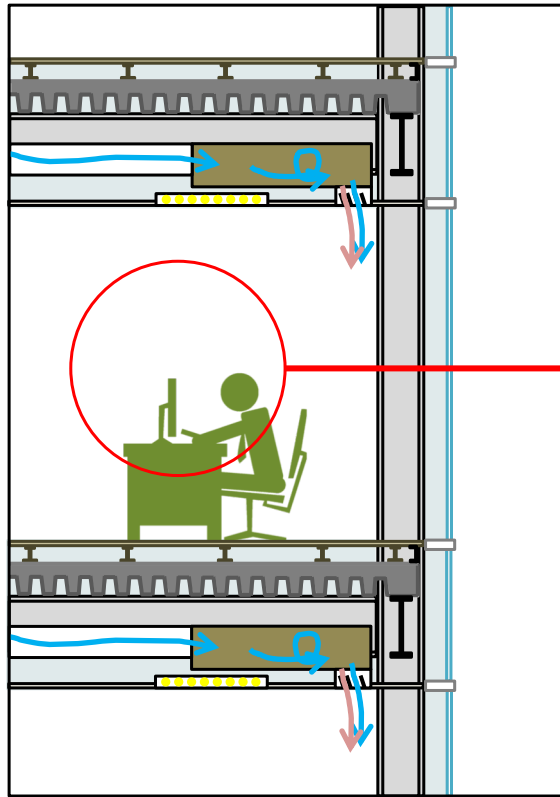
Glass Façade Full A/C
